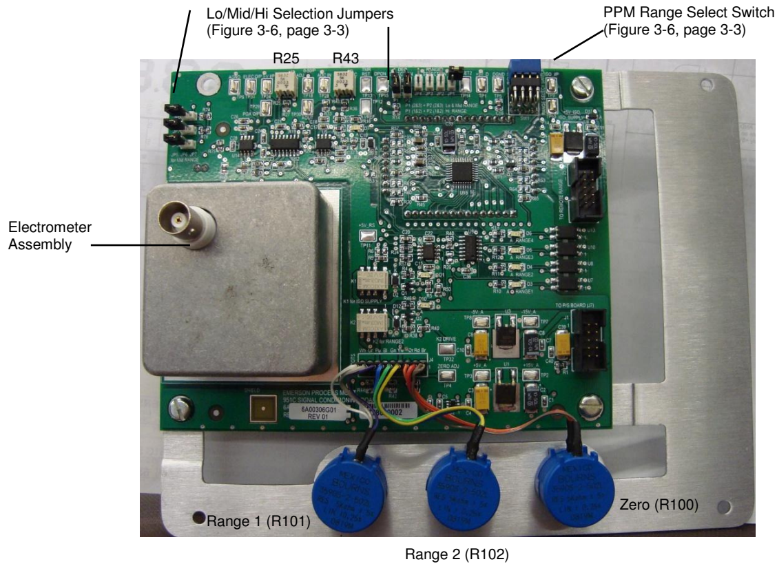
Figure 3-2. Signal Board
